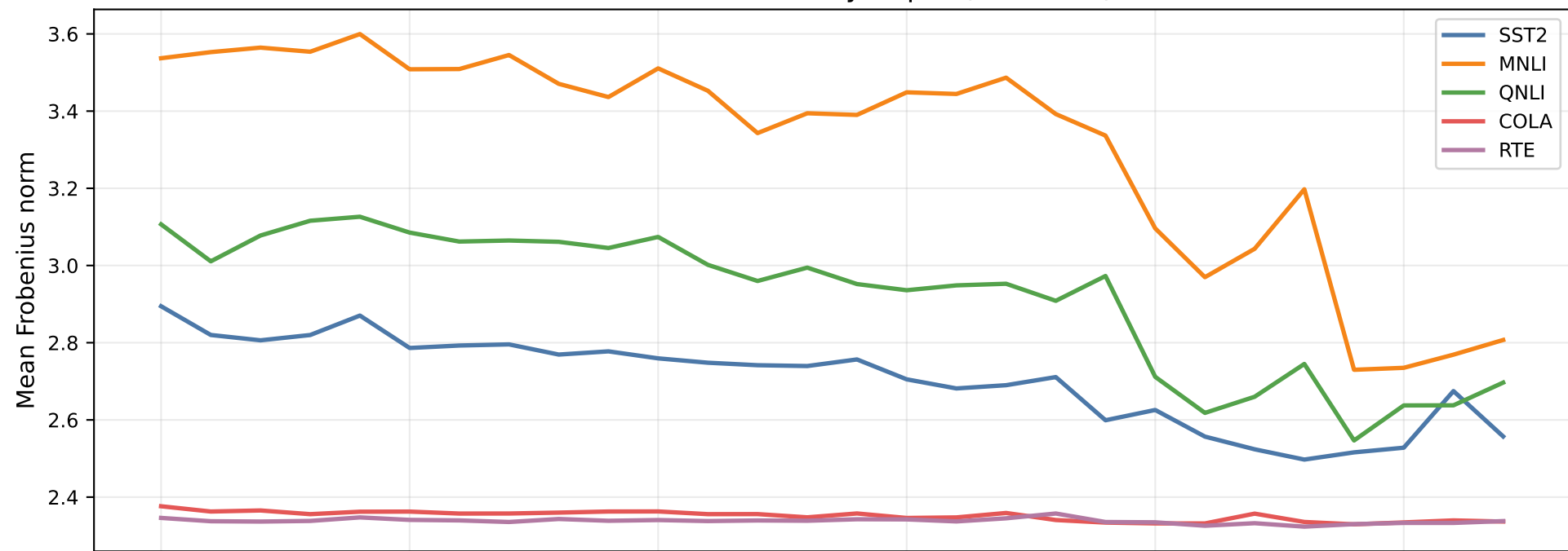
Mean LoRA A norm by depth (mlp)
