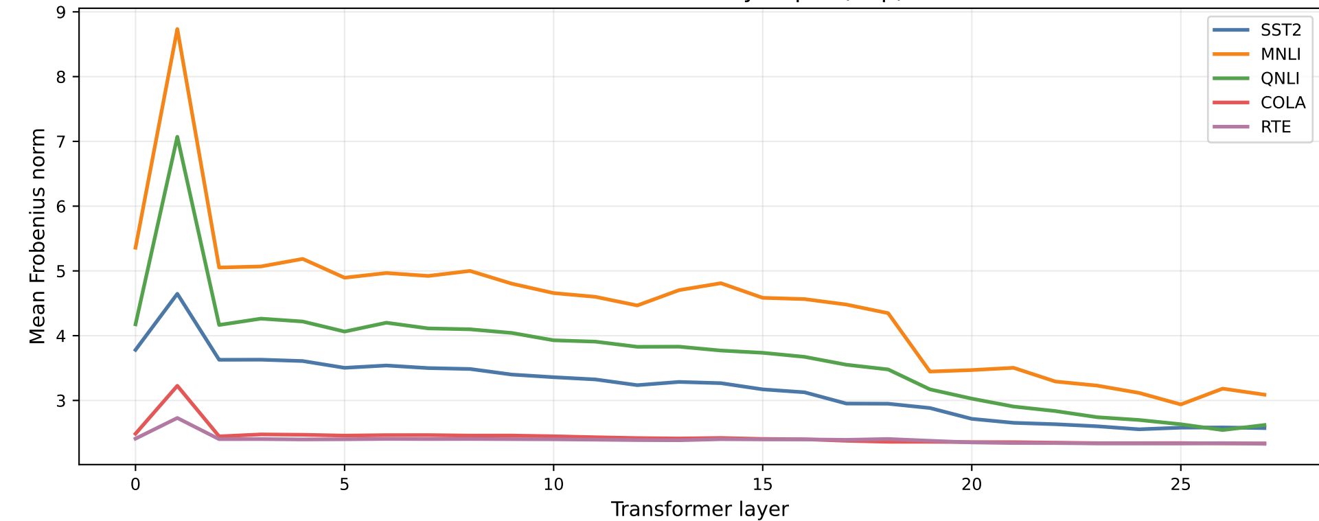
Mean LoRA A norm by depth (mlp)
